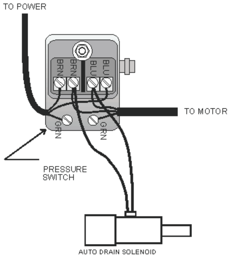
INSTALLATION WIRING DIAGRAM
