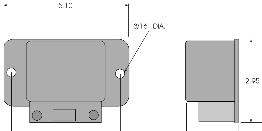
OUTLINE, AUTO ISOLATOR I CONTROLLER, 091-208-12
