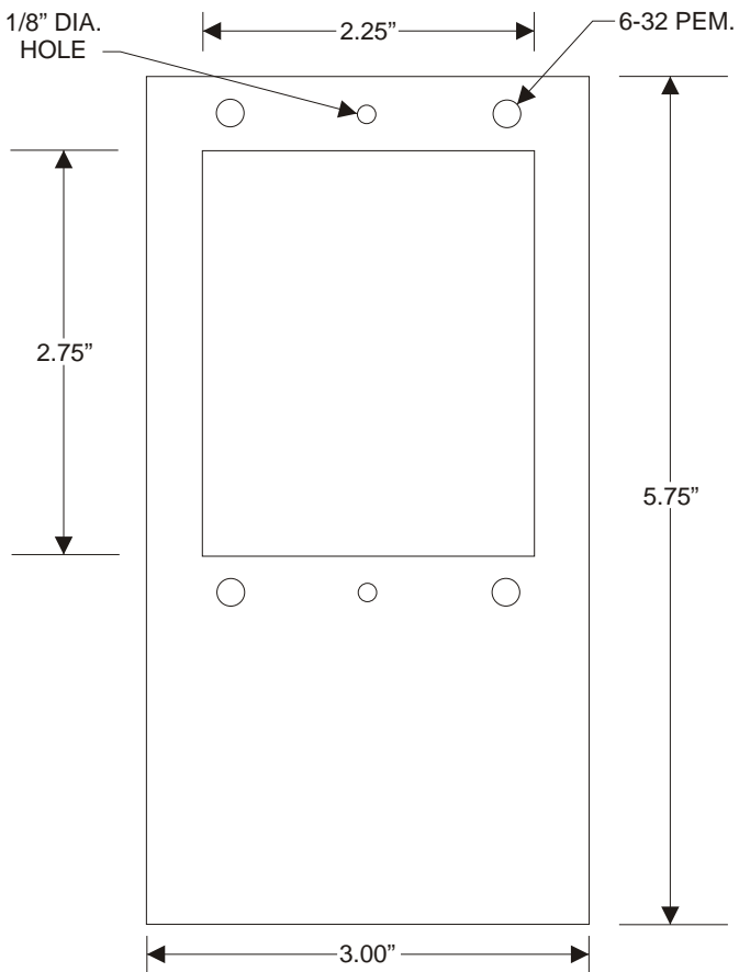
MODEL # 091-18CP OUTLINE DRAWING
