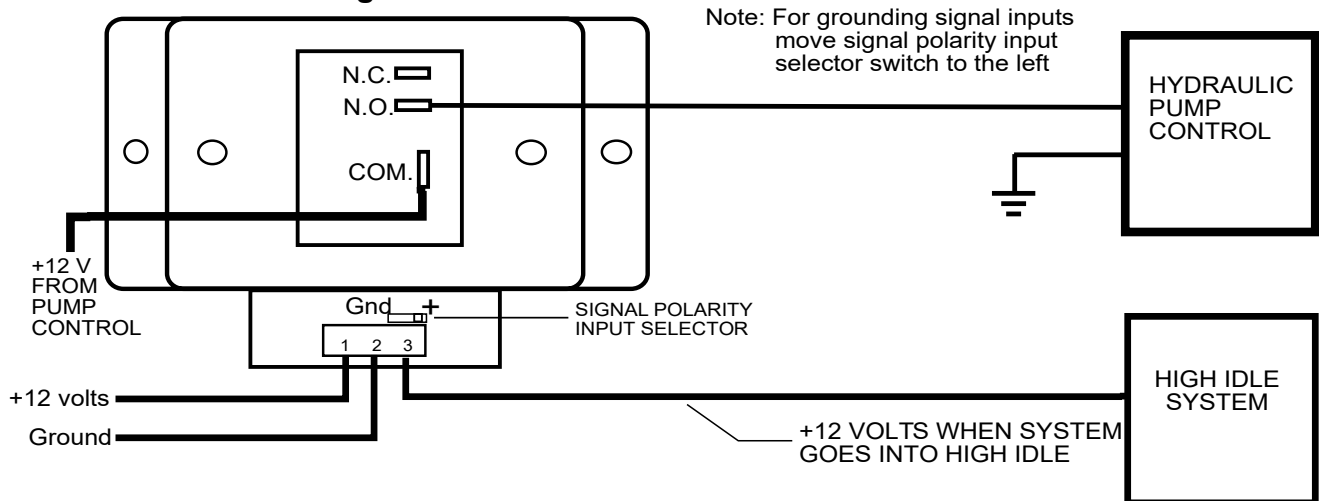
TYPICAL INSTALLATION WITH HIGH IDLE PRECEDING HYDRAULIC PUMP START UP
