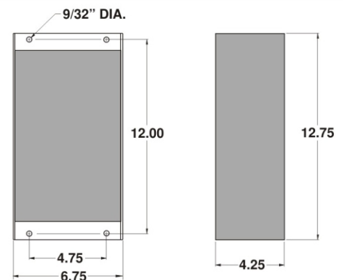
091-170-DV-12 Outline Drawing
