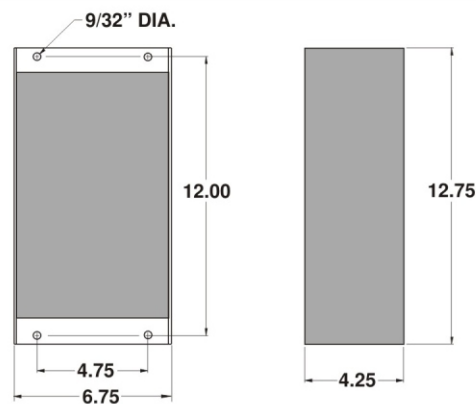
091-170-12 Outline Drawing
