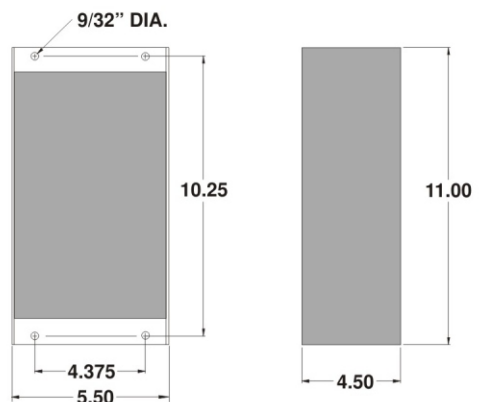
091-165-12 Outline Drawing
