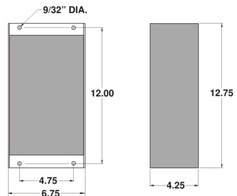
091-11HO-12 Outline Drawing
