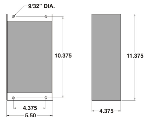
091-11DV-12 Outline Drawing
