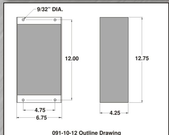
091-10-12 Outline Drawing
